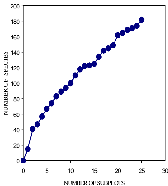
Figure 2. Species-area curve for trees with DBH ≥ 10 cm in a one-hectare plot of a lowland forest at the Batang Gadis National Park, North Sumatra, by plotting the number of species against the number of subplots of 20x20 m each.
