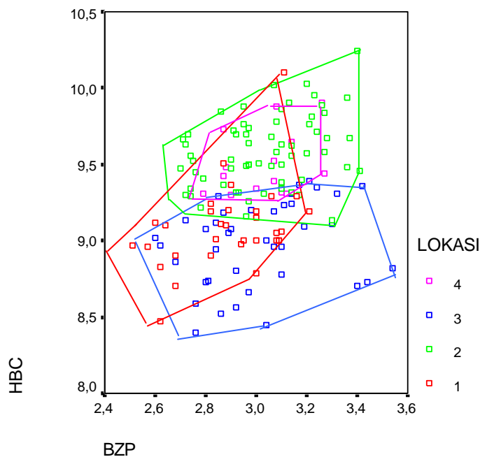
Figure 3. Bivariate plot of HBC and BZP of Maxomys whiteheadi from Kalimantan. (1) Gunung Palung and Tanjung Putting (West Kalimantan); (2) Sebangau and Barito Ulu (Central Kalimantan); (3) Bukit Bangkirai (East Kalimantan) and (4) Kayan Mentarang (North East Kalimantan).
